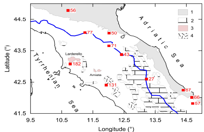
Figure 5 - Heat flow values (in \text{mW m}^{-2} ) as inferred from selected thermal data of deep boreholes (see also Table 2). The Apennines watershed is also indicated (blue line). Details as in Fig. 1.
