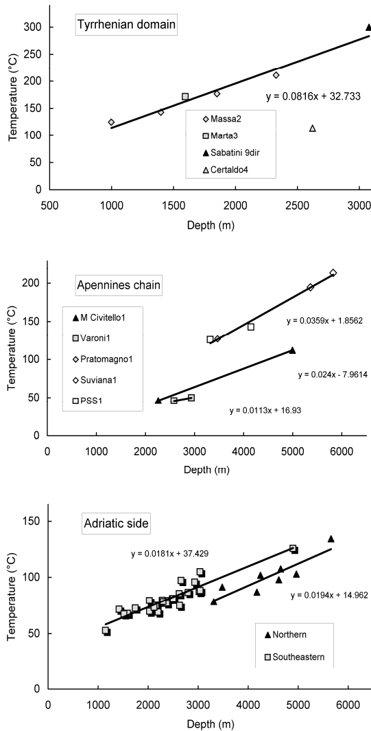
Figure 3 - Plot of the corrected temperature vs. depth of the wells reported in Table 1 of the Tyrrhenian domain and the Adriatic domain: Apennines chain, northern sector and southeastern sector of the Adriatic side. Temperature depths are referred to the sea level.
